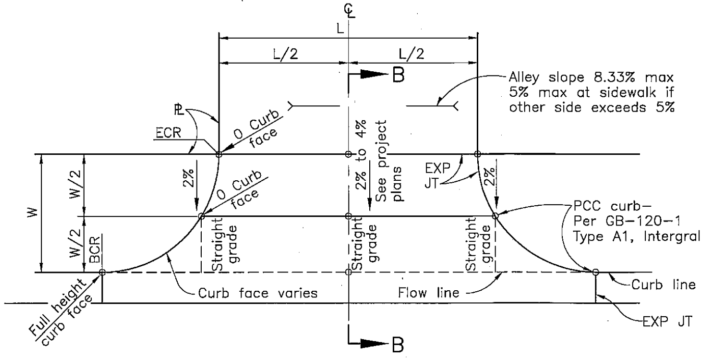
PLAN W = 1.8 m (6') TO 2.7 m (9')
