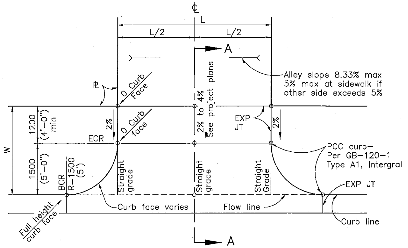
PLAN W = 2.7 m (9') OR GREATER
