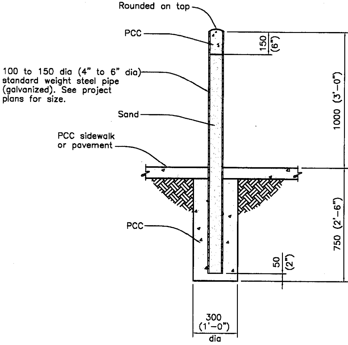
TYPICAL SECTION
