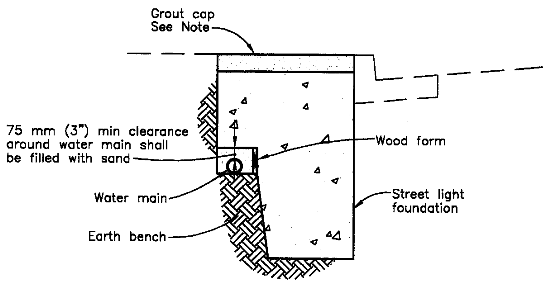
DETAIL B
