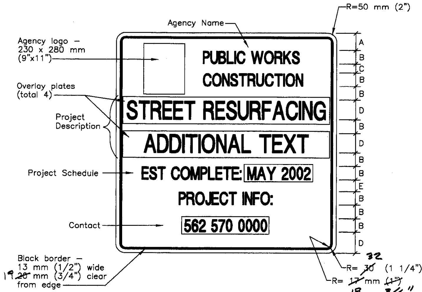
1220 x 1220 mm (48"x48") SIGN
